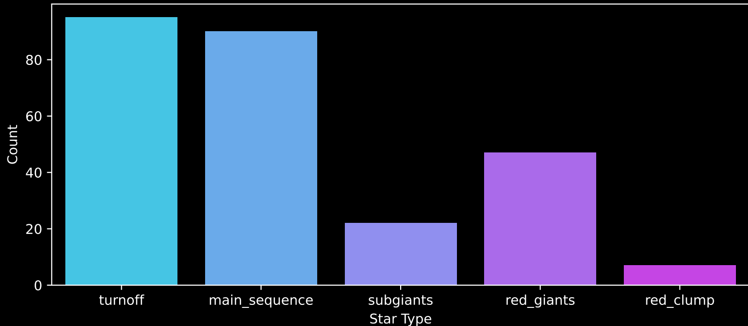
GALAH DR4 Field: [2600] Count plot of Star Type
