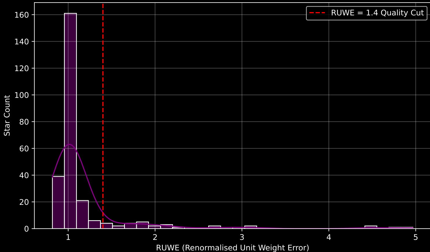
GALAH DR4 Field [2600] RUWE Distribution (n= 257)
