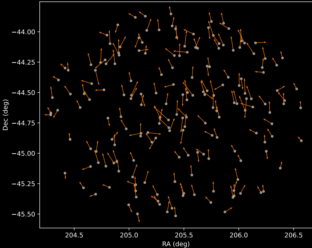
GALAH DR4 Cluster 2 Proper Motion Vectors (n=185)
